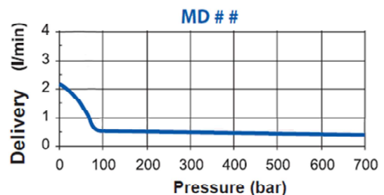
Oil Delivery Flow Chart
